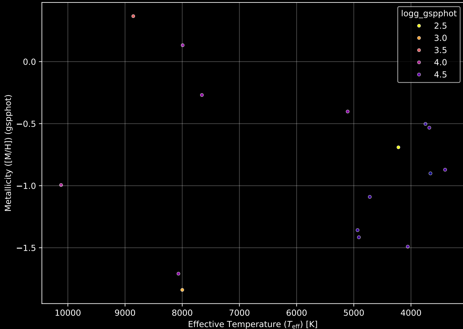
APOGEE DR17 Field: [358+00-C] Stellar Population Parameters (n= 16)
