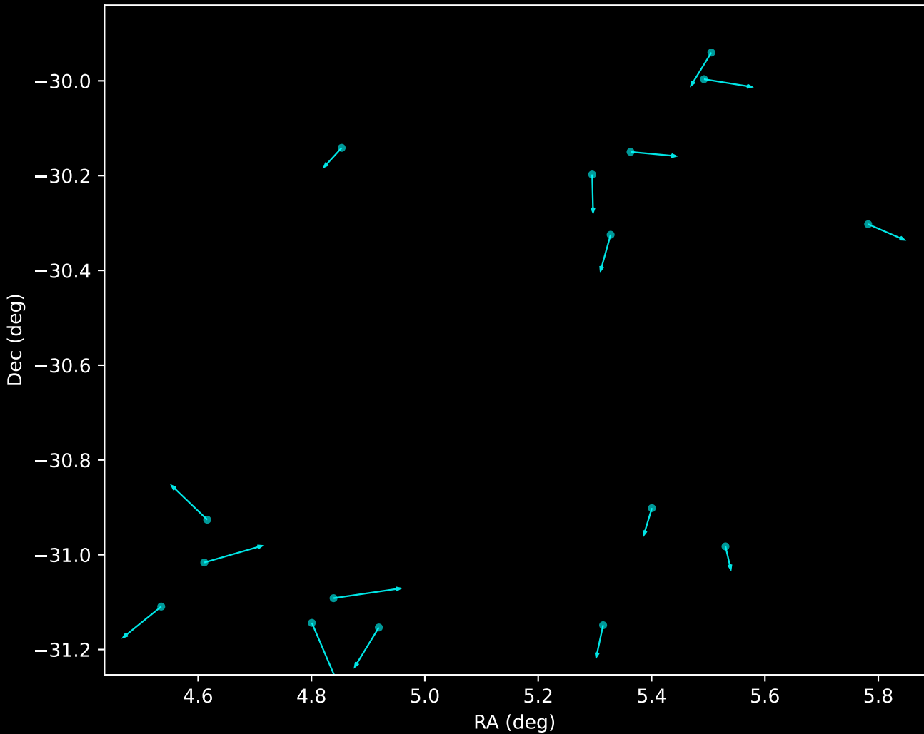
APOGEE DR17 Noise Stream Proper Motion Vectors (n=16)
