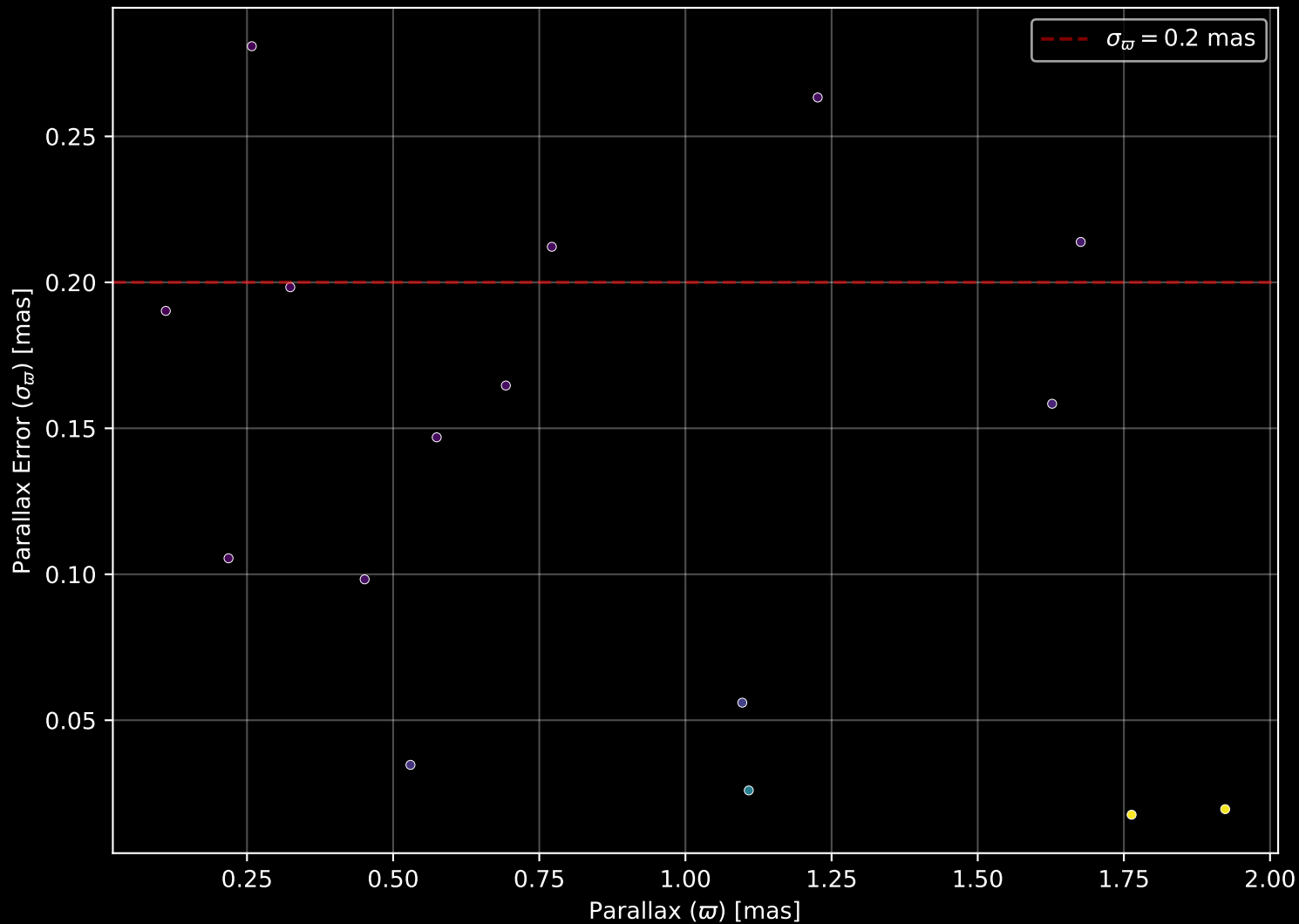
APOGEE DR17 Field: [358+00-C] Parallax Quality (n= 16)
