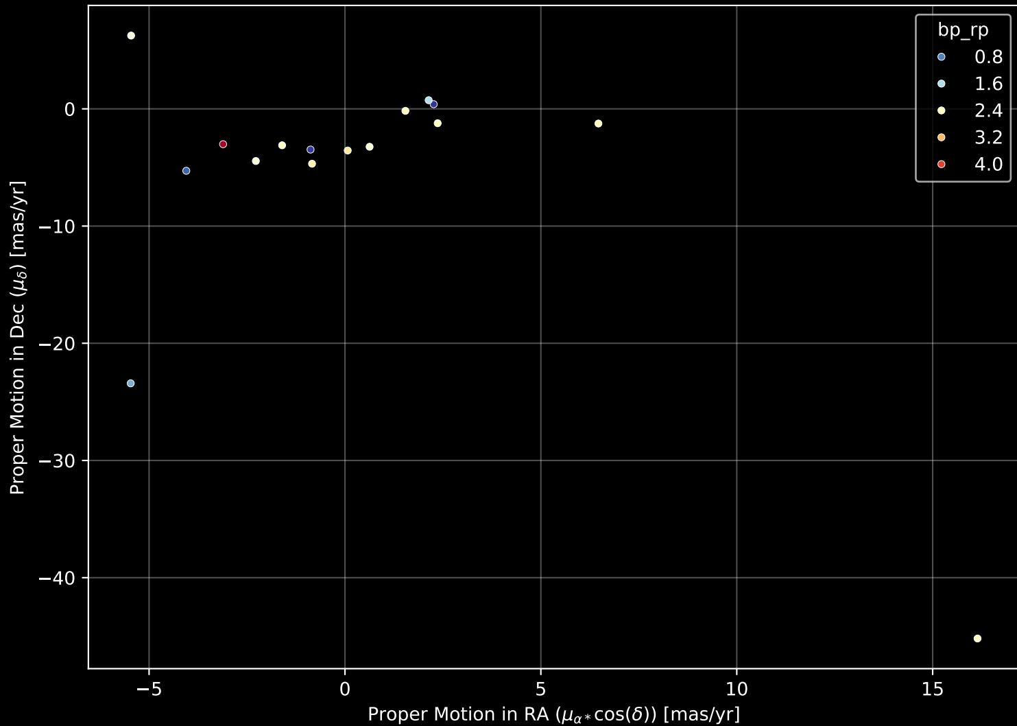
APOGEE DR17 Field: [358+00-C] Proper Motion Diagram (n= 16)
