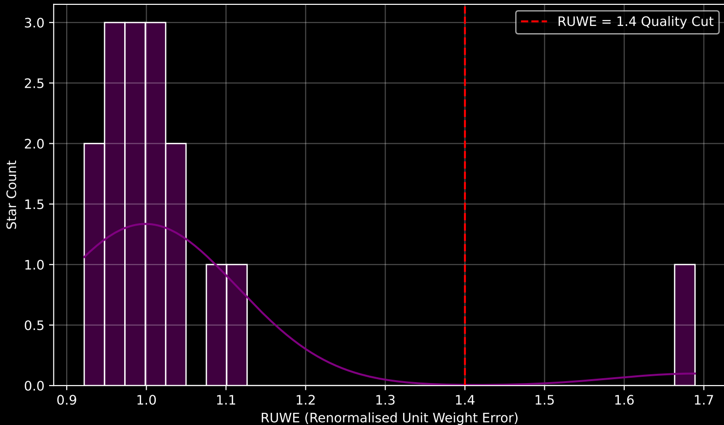
GAPOGEE DR17 Field [358+00-C] RUWE Distribution (n= 16)
