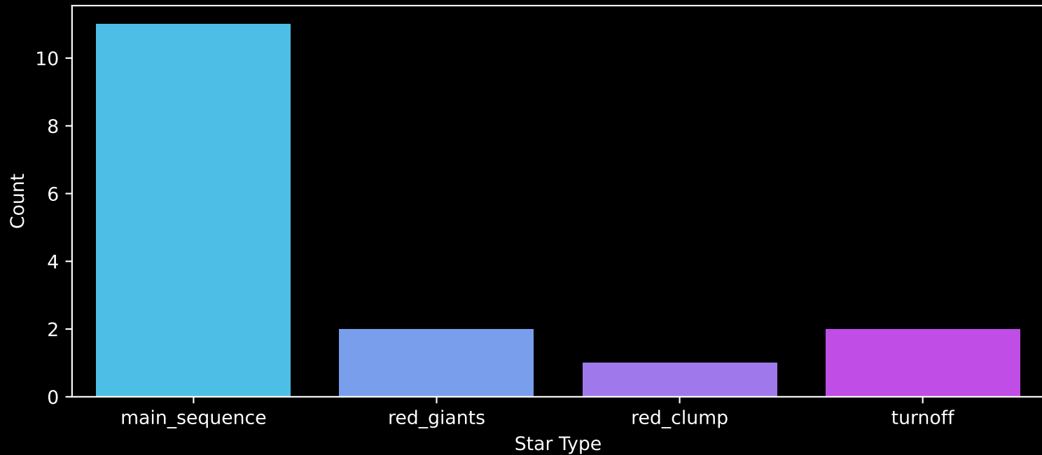
APOGEE DR17 Field: [358+00-C] Count plot of Star Type
